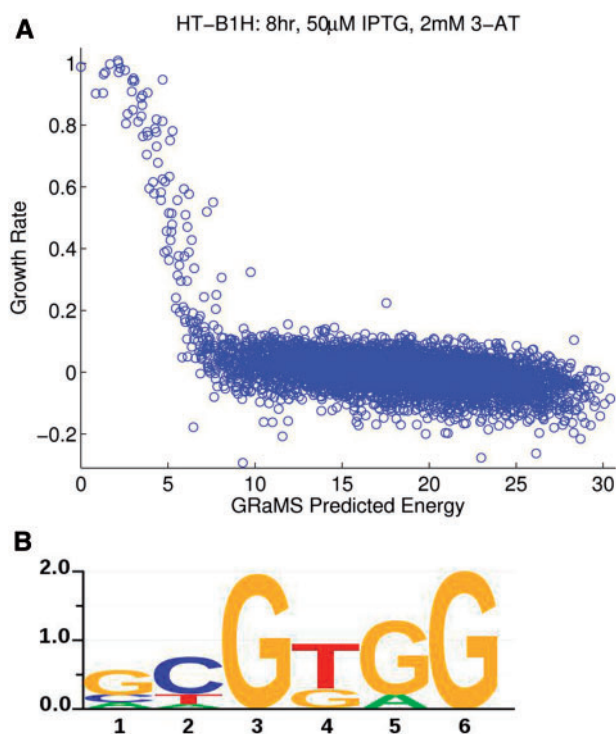
Figure 3. Results of CV-BIH on Zif268 analyzed with GRaMS. (A) Plot of predicted energies versus growth rates per 6-mer. The GRaMS PWM (8 h, 50 \mu M IPTG, 2 mM 3-AT) was used to predict the energies. The growth rates (shifted so that the median value is zero) are from the 8 h, 50 \mu M IPTG, 2 mM 3-AT data set used to estimate the GRaMS PWM. (B) Sequence logo for the GRaMS PWM obtained from the same data set. The y-axis indicates the information content of each position in bits. Sequence logos were produced using in-house software, svgSeqLogo , written by RGC.
