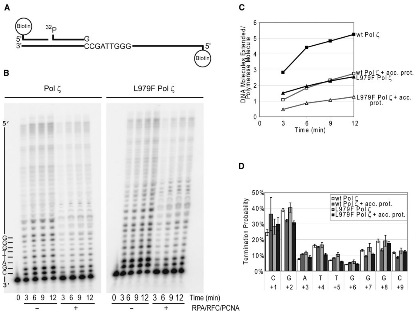
Figure 2. Catalytic activity of wild-type and L979F Pol \zeta . (A) Substrate. The substrate consists of a 70-mer template oligonucleotide with a 5'-biotin moiety, to which were annealed a 14-bp oligonucleotide with a 5' biotin moiety and a ^{32}\text{P} -labeled 16-bp primer without a biotin moiety. Streptavidin was used to block substrate ends. (B) Primer extension assay. Eight- and five-fold excess substrate over enzyme were used for wild-type Pol \zeta and L979F Pol \zeta , respectively. Under these conditions, each substrate molecule is encountered by a polymerase molecule only once. Where indicated, PCNA, RFC and RPA were loaded onto the substrate and incubated for 2 min, and then polymerase was added to start the reactions. Time points were taken at 3, 6, 9 and 12 min. A portion of the template sequence is shown at the left. (C) Primer extension activity. The number of DNA molecules extended per polymerase molecule is plotted against time. Acc. prot. indicates presence of accessory proteins PCNA, RFC and RPA. (D) Termination probabilities at each template position. The termination probabilities shown are an average of the four time points shown in (B), with the error bars indicating the standard deviations between the time points.
