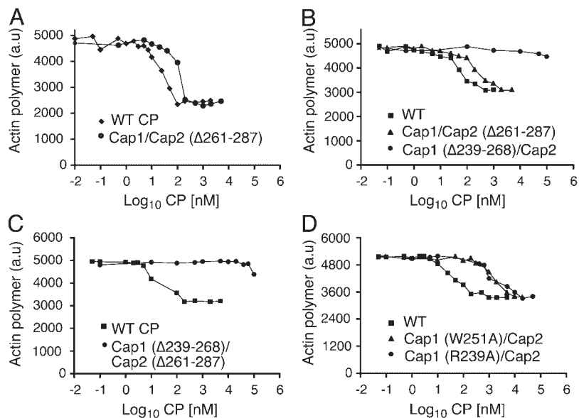
Figure 5. Effect of CP mutants on the apparent critical concentration for actin polymerization at steady state. Pyrene actin fluorescence intensity, reflecting polymerized actin, is plotted vs. the log of the CP concentration. CP mutants are as indicated on each panel.
