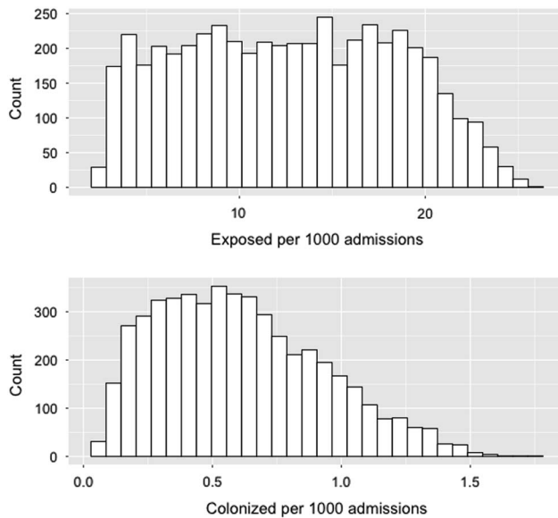
FIGURE 2. Histograms for the simulated number of patients exposed to Clostridium difficile in food and colonization events due to exposure to C. difficile spores in food. Counts are the number of exposed and colonized patients in each histogram bar.
