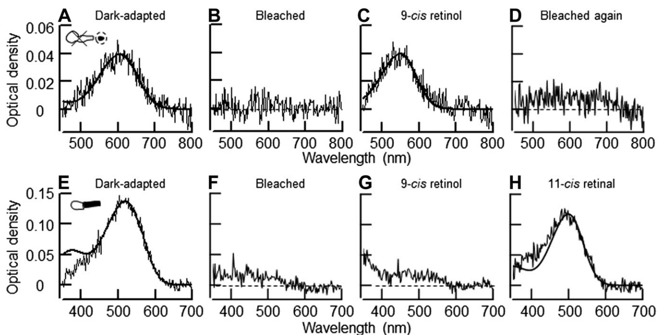
Fig. 4. Microspectrophotometric measurement of pigment regeneration in a truncated cone outer segment and in an intact rod. (A) Absorbance spectrum of a dark-adapted cone outer segment. Fitted to the data is a visual pigment template with peak wavelength at 605 nm and an optical density of 0.039. (B) Absorbance spectrum of the same cone outer segment as in (A) recorded after >99% of the visual pigment had been bleached. (C) Absorbance spectrum of the same bleached cone outer segment as in (B) recorded after treatment with 9- cis retinol. Fitted to the data is a visual pigment template with peak wavelength at 549 nm and an optical density of 0.040. (D) Absorbance spectrum of the same regenerated cone outer segment as in (C) recorded after a second >99% bleach of its visual pigment. (E) Absorbance spectrum of the outer segment of an intact dark-adapted red rod. Fitted to the data is a visual pigment template with peak wavelength at 518 nm and an optical density of 0.14. (F) Absorbance spectrum of the same rod as in (E) recorded after >99% of the visual pigment had been bleached. (G) Absorbance spectrum of the same bleached rod as in (F) recorded after treatment with 9- cis retinol. (H) Absorbance spectrum of the same bleached rod as in (G) recorded after treatment with 11- cis retinal. Fitted to the data is a visual pigment template with peak wavelength at 500 nm and an optical density of 0.12.
