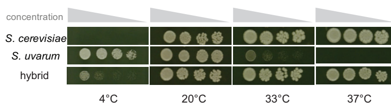
FIG. 1. —Temperature dependent growth of Saccharomyces cerevisiae , S. uvarum and their hybrid. Growth is after 17 days at 4°C, 3 days at 20°C and 2 days at 33°C and 37°C, with platings on YPD at 1:3 serial dilutions.
