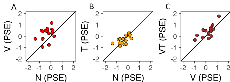
Figure 3. Planned comparisons on PSE values Each point corresponds to PSE estimates for a single participant. (A) Comparison between the baseline condition (N) containing no surround orientation information and the visual-only condition (V). (B) Comparison between the baseline condition and the tactile-only condition (T). (C) Comparison between the visual-only condition and the visuo-tactile condition (VT). Points above the unity line indicate subjects exhibiting larger repulsive tilt illusion effects in the condition plotted on the ordinate compared to the abscissa.
