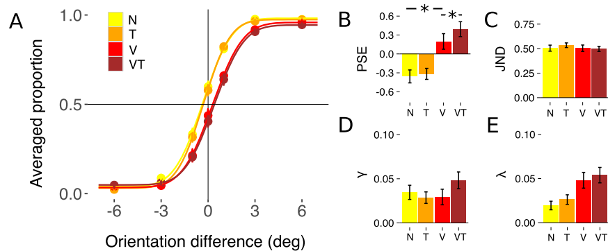
Figure 2. Orientation discrimination performance (A) Group averaged choice probability data and group level psychometric functions for each surround condition (None, Tactile-only, Visual-only and Visuo-tactile). Mean of the group distribution of individual PSE (B) JND (C) \gamma (D) and \lambda (E) parameters. Error bars represent standard error. Asterisks represent those hypothesis-driven contrasts that showed a significant effect.
