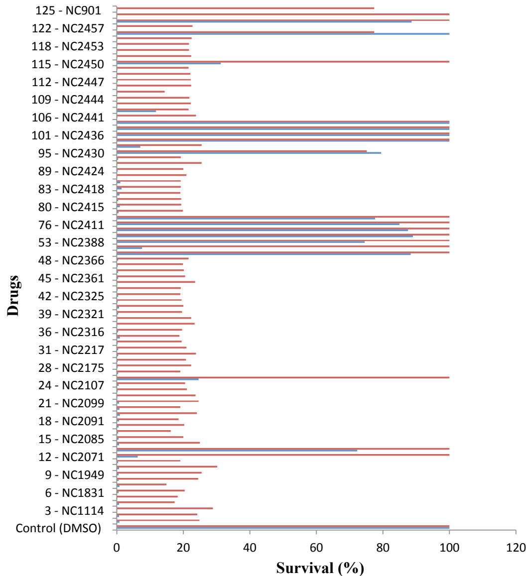
Figure S1. Screening of the enone library of 126 compounds. Evaluation of anti-leishmanial (blue line) and cytotoxic activity to mammalian cells (LLC-MK2 - red line) after 96 h of incubation with the compounds. The criteria used to identify potential hits were the observance of less than 75% survival of L. major promastigotes (blue) and greater than 75% survival in LLC-MK2 cells (red). Six compounds met this initial criteria.
