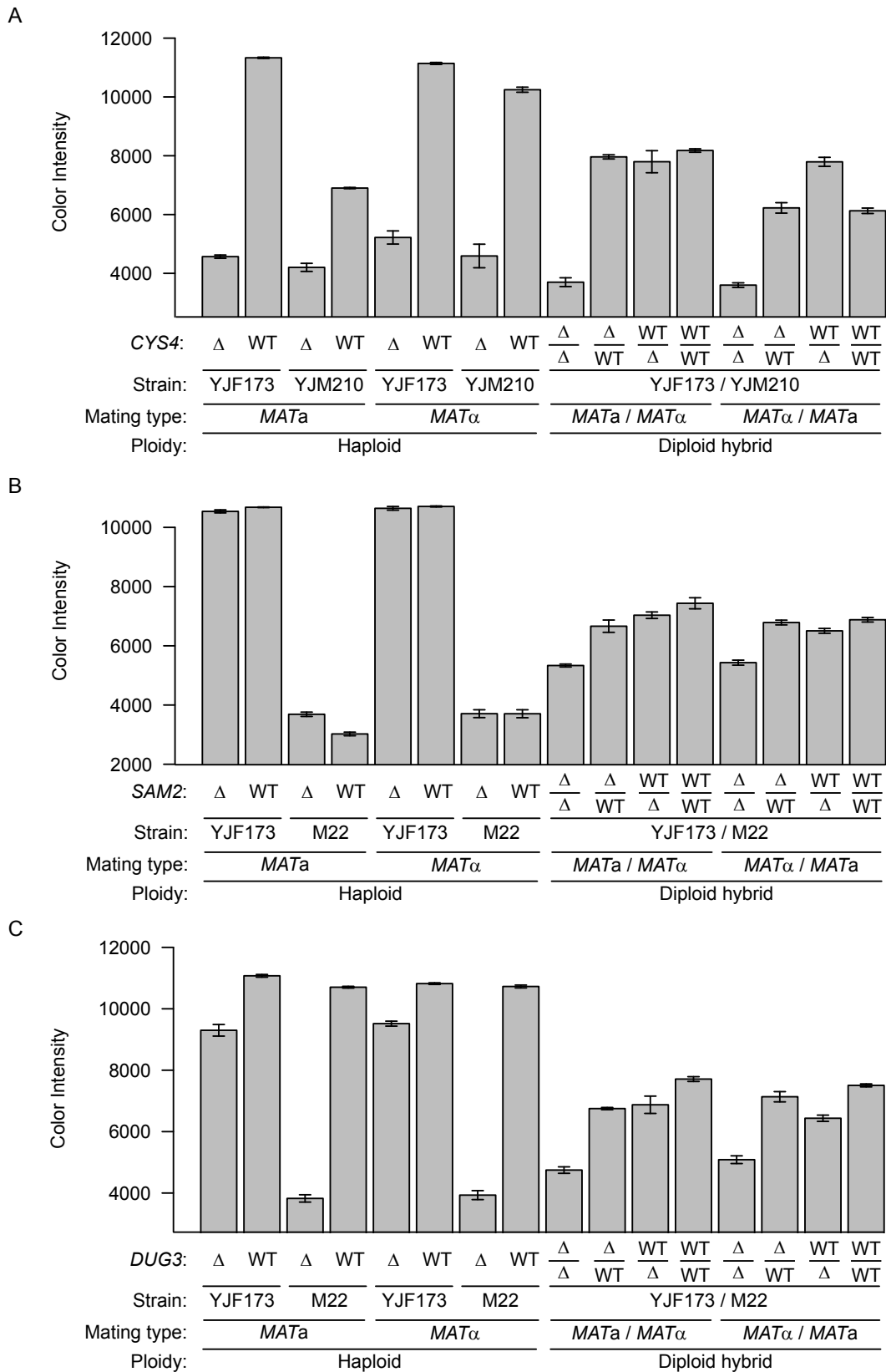
Figure S4 Phenotypes of strains used for the replicated reciprocal hemizyosity analysis. (A) Effects of CYS4 on colony color. (B) Effects of SAM2 on colony color. (C) Effects of DUG3 on colony color. Each panel shows mean and standard error (bars) of colony color for strains with different: ploidy, mating type, strain background and genotype at either CYS4 , SAM2 or DUG3 , where \Delta indicates a deletion and WT indicates the wild-type strain allele.
