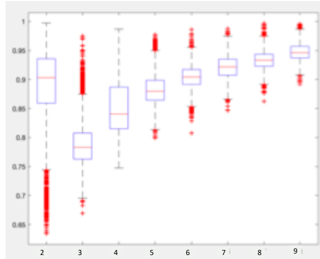
Concordance Index
