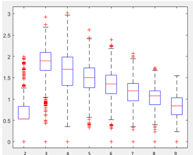
Variation of Information
