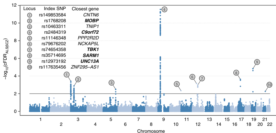
Figure 4 | Pleiotropy-informed ALS risk loci determined by analysis of cFDR in ALS GWAS P-values given schizophrenia GWAS P-values ( cFDR_{ALS|SCHZ} ). Each point denotes a SNP; its x axis position corresponds to its chromosomal location and its height indicates the extent of association with ALS by cFDR analysis. The solid line indicates the threshold cFDR = 0.01. Any gene whose role in ALS is already established is in bold. A complete list of all loci at cFDR ≤ 0.05 is provided in Supplementary Table 8.
